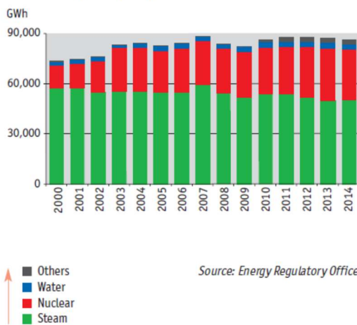
Chart 1 → Electricity generation by power plant type in the Czech Republic [GWh], 2000–2014
